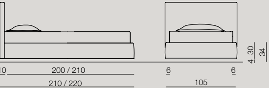
Materasso L90 x P190/200 cm. / Mattress W90 x L190/200 cm.
