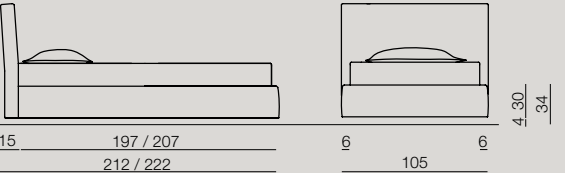
Materasso L90 x P190/200 cm. / Mattress W90 x L190/200 cm.
