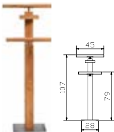
Herrendiener | valet | dressboy Claudio alu, anthracit, iron
